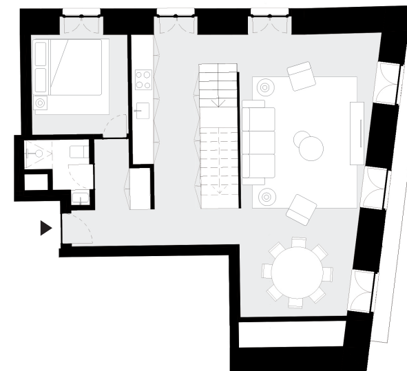
PISO 2 floor 2
