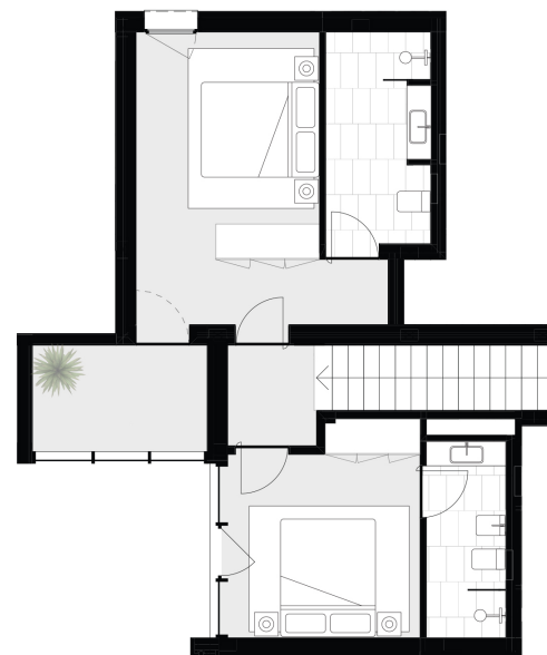
PISO 1 floor 1
