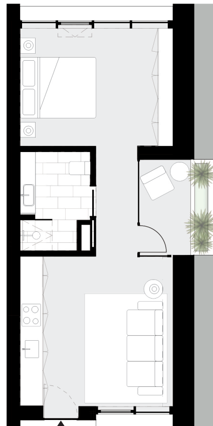
PISO 3 floor 3
