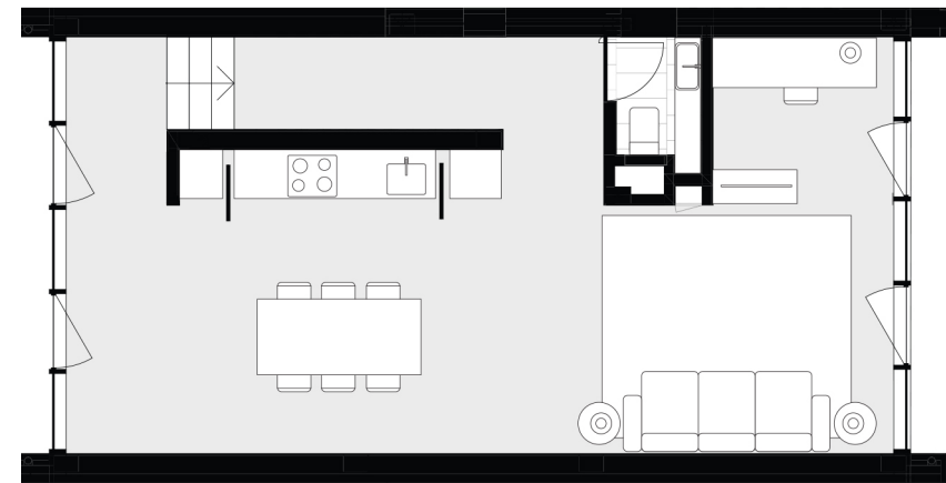
PISO 1 floor 1
