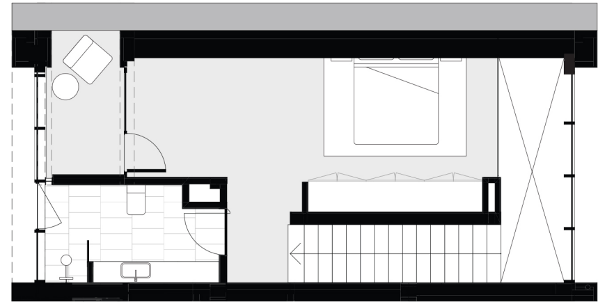
PISO 2 floor 2
