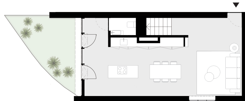
PISO 0 floor 0
